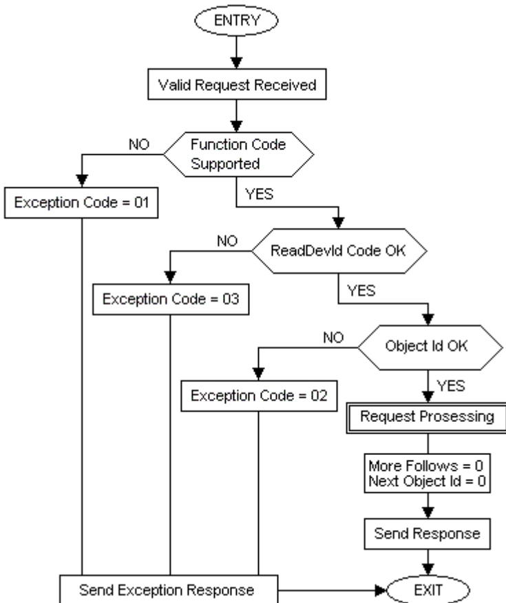
Figure 11, Read Device Identification state diagram
