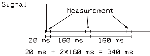
Figure 27, signal measurement in Security Module
