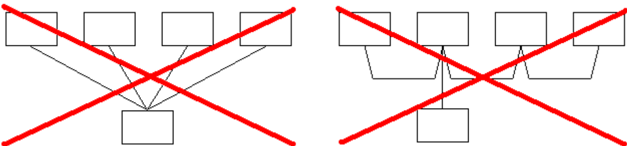
Figure 2, Wrong way to connect RS-485 bus
